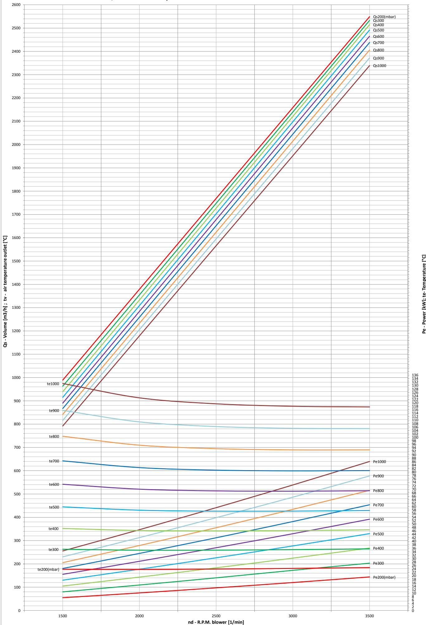
KTSR180 -Volume Flow Rate, Power and Air Temperature in Outlet Vs R.P.M for Pressure Difference 200 - 1000 mbar
