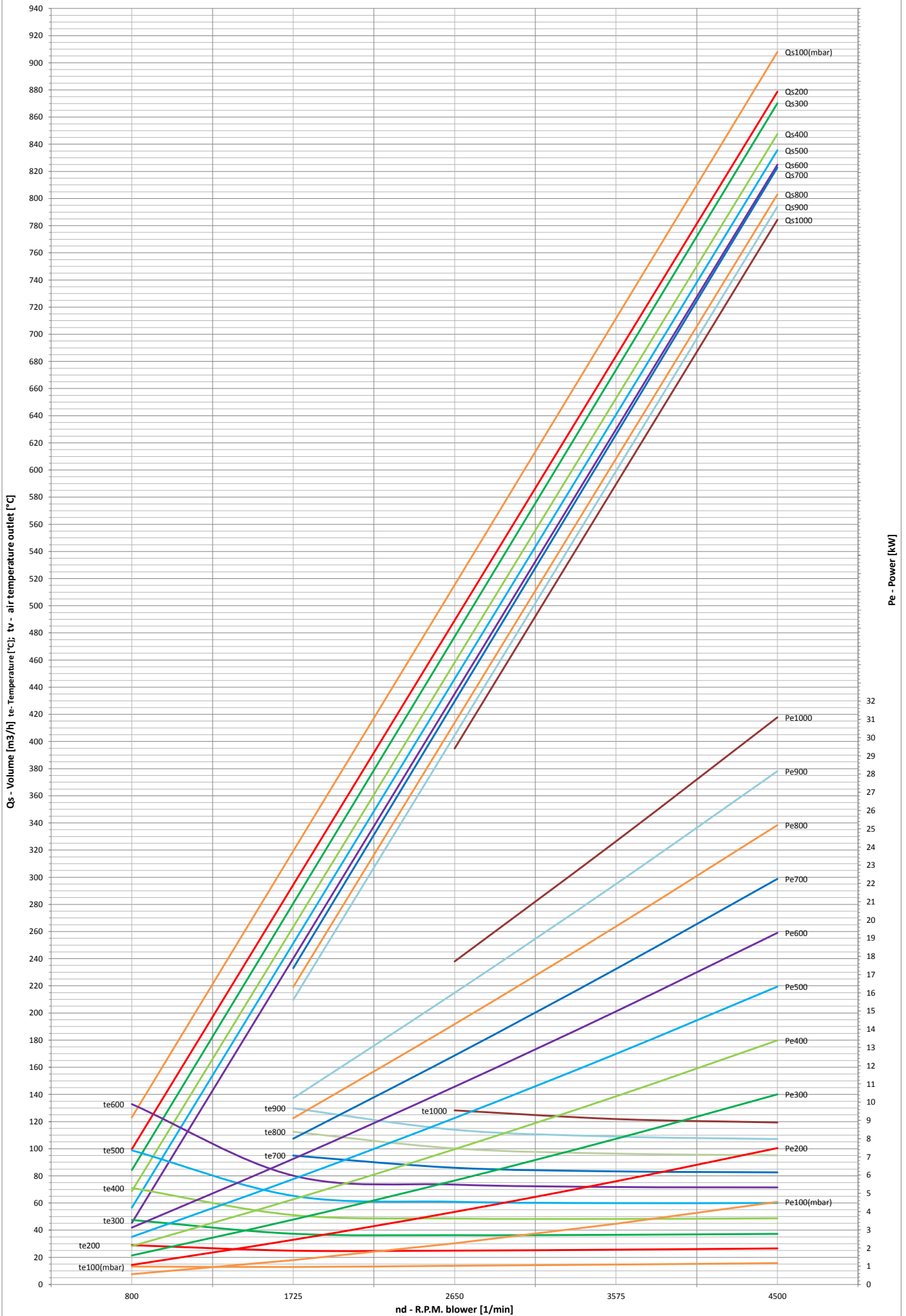
KTSR50 - Volume Flow Rate, Power and Air Temperature in Outlet Vs R.P.M for Pressure Difference 100 - 1000 mbar
