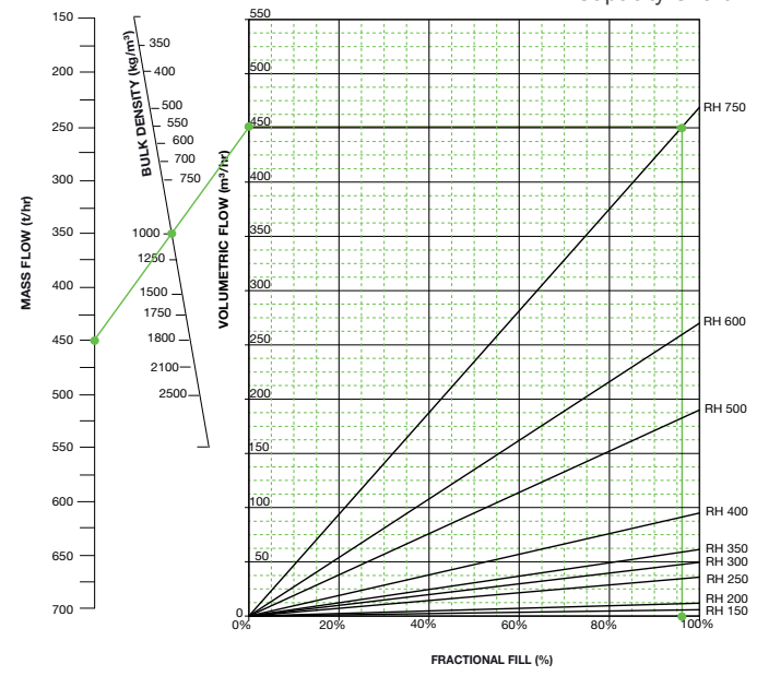
Capacity Chart
