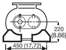
VERTICAL AIRFLOW BLOWER (for other dimensions see below)
