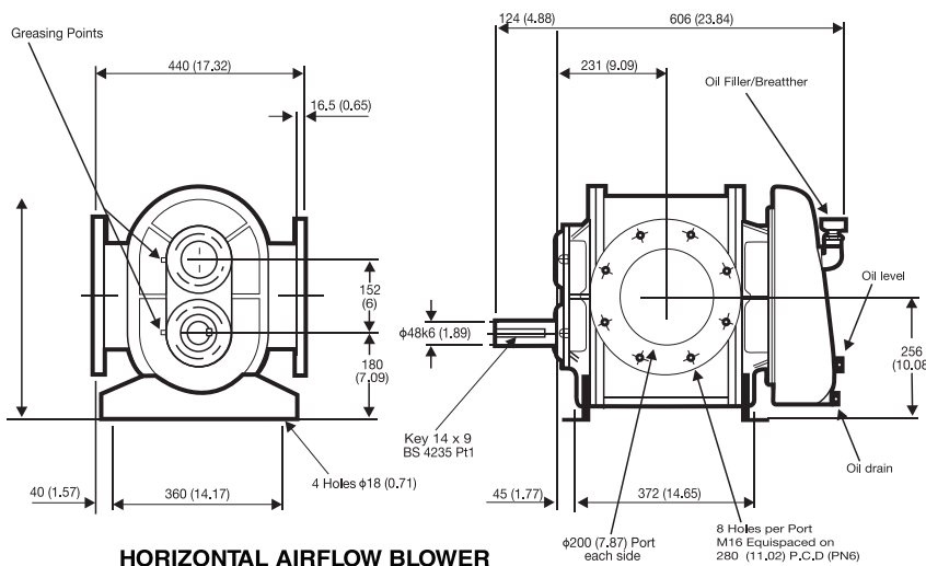
HORIZONTAL AIRFLOW BLOWER
